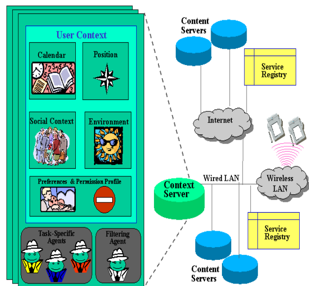
Fig. 1 Overview of MyCampus Architecture
